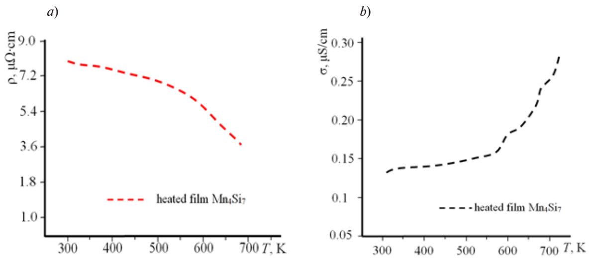
Fig. 4. Temperature dependences of the resistivity (a) and electrical conductivity (b) of the \text{Mn}_4\text{Si}_7 annealed film in polycrystalline phase
