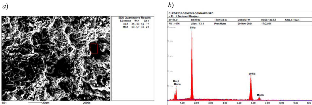
Fig. 1. The results of studying the Mn 4 Si 7 target with a scanning electron microscope (SEM): the surface image (a) and energy dispersive X-ray spectrum (b)
