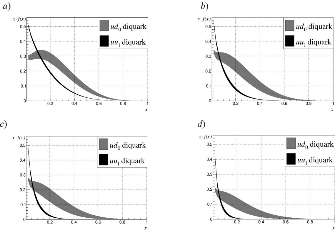
Fig. 1. Graphs of the x:f(x) functions (diquark PDFs) at different scale energies \mu^2 , (GeV) 2 : 10 (a), 10 2 (b), 10 3 (c), 10 4 (d). The cases of the scalar ud_0 (gray bands) and vector uu_1 (black ones) diquarks are shown
