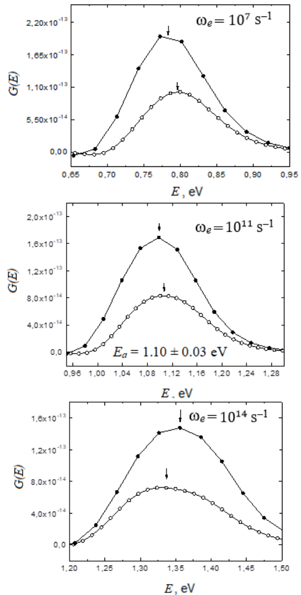
Fig. 6. The data similar to those shown in Fig. 5 but for HIPS with 6 vol.% of \text{TiO}_2 ; E_a = 1.10 \pm 0.03 eV
